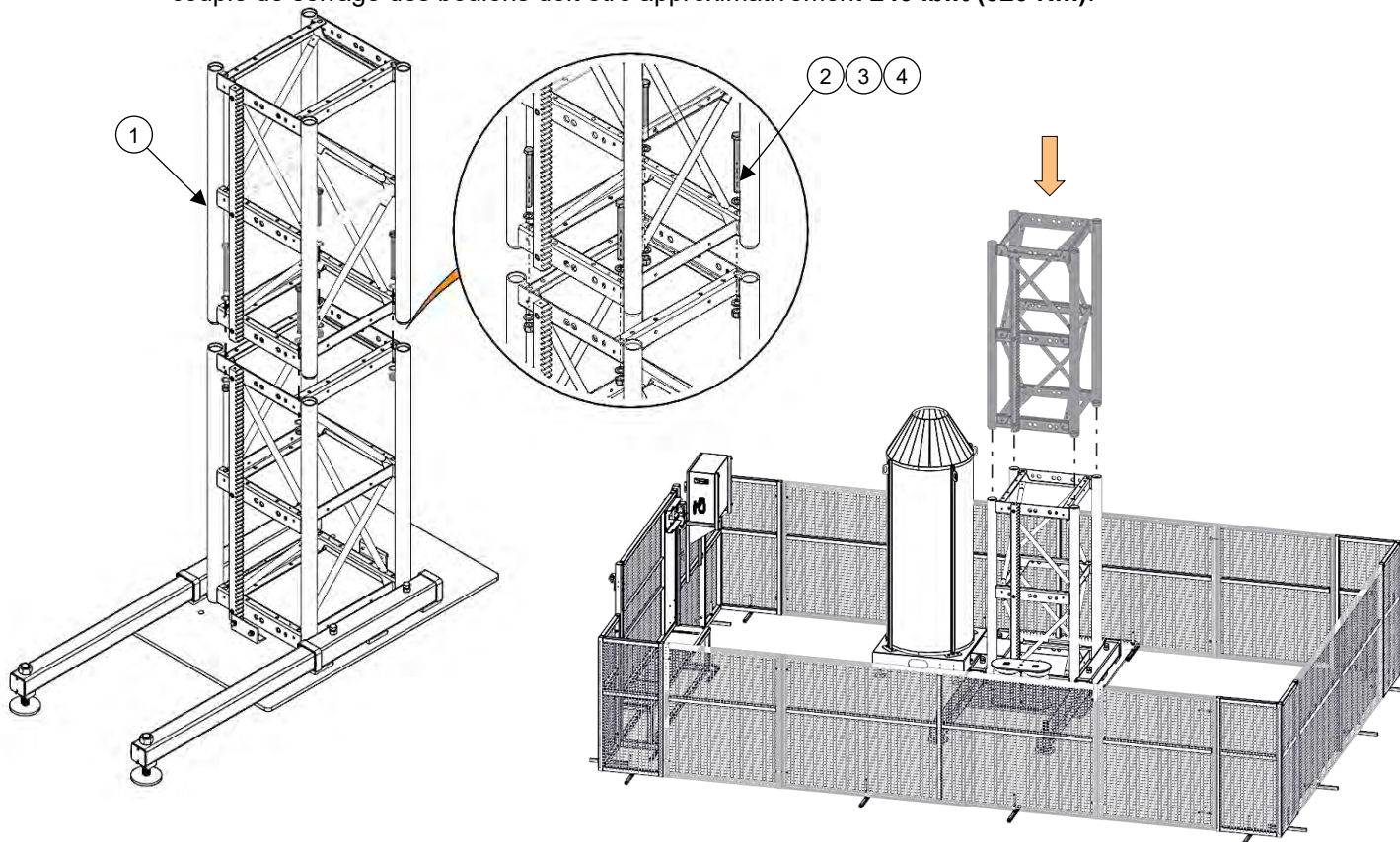
Figure 8 - Installation des sections de mât
